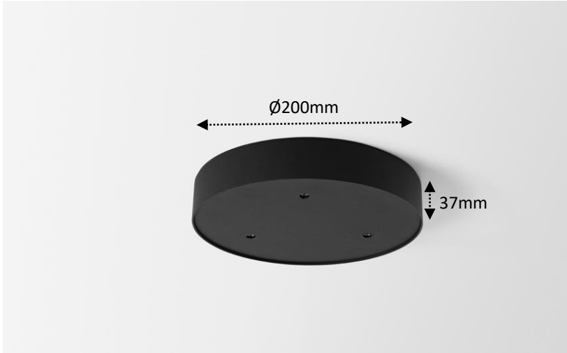
Round For 3x jack (WD) Black struc / white struc
