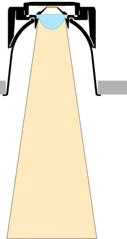
ASPHERICAL LENS 30° Projected light LED 984 lm 622 lux in the center at 2m
