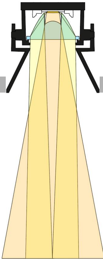
TIR LENS 25° Total inner reflection LED 712 lm 753 lux in the center at 2m
