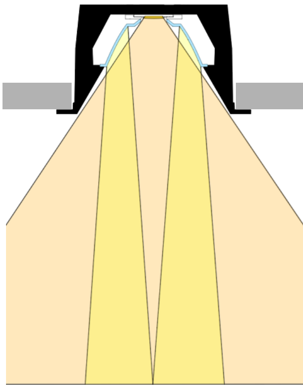
REFLECTOR 25° direct light + reflected light LED 773 lm 589 lux in the center at 2m
