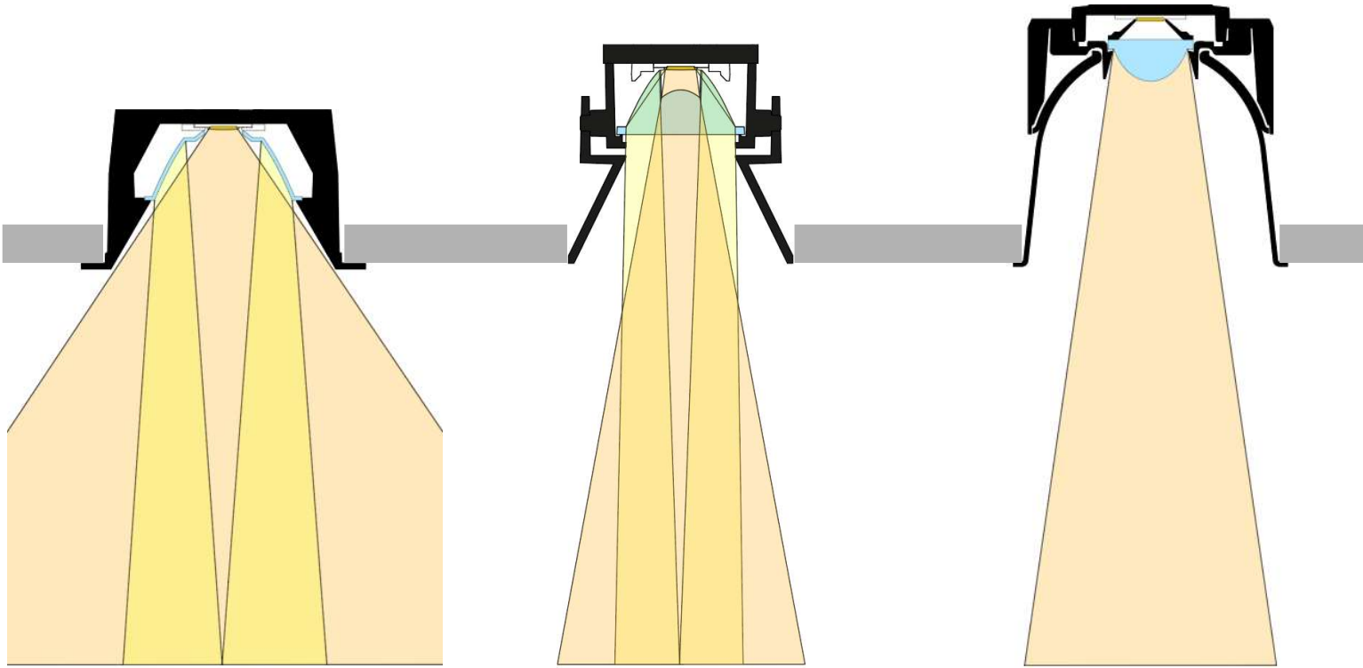
REFLECTOR 25° direct light + reflected light LED 773 lm 589 lux in the center at 2m
